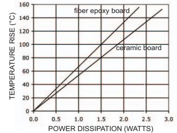
POWER DERATING
