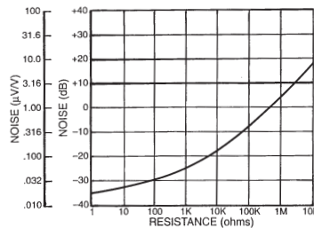
CURRENT NOISE
